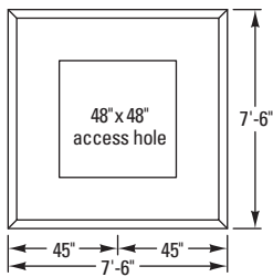
Frost box concrete pad
