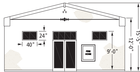
West portico elevation
