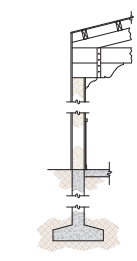
Section through wall
