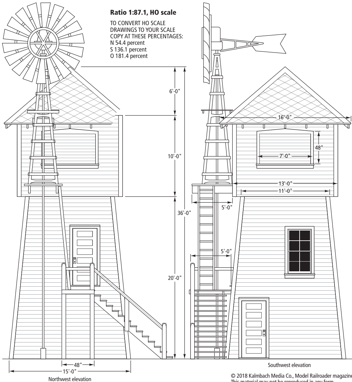
Northwest elevation
